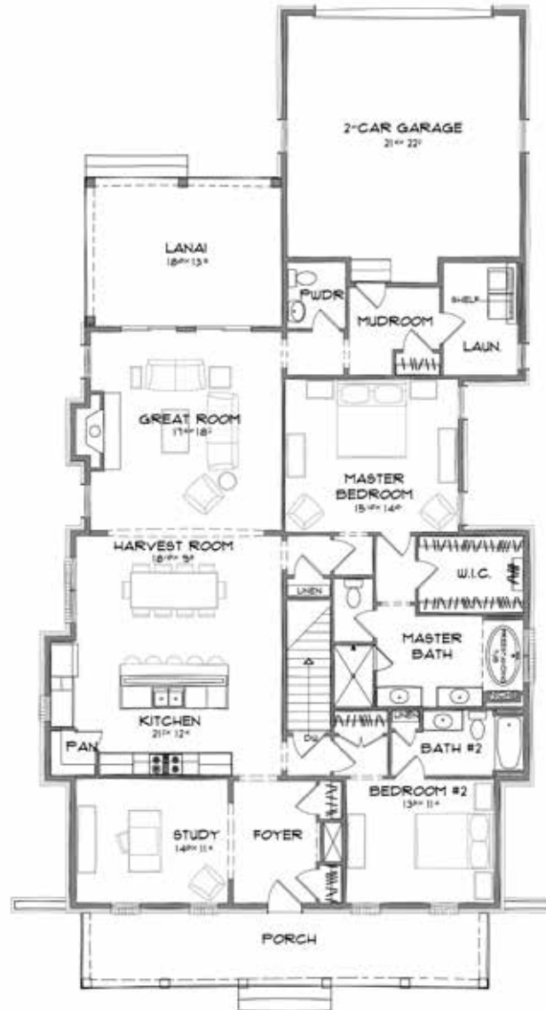
Main Level
